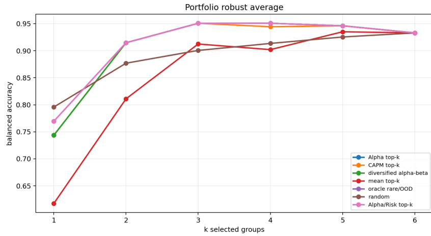
Figure 5: Synthetic robust-average group acquisition. The y -axis averages balanced accuracy over rare, OOD, and spurious-shift slices.
