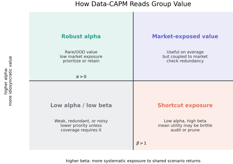
Figure 1: Conceptual diagnostic map. Positive alpha suggests value beyond the shared scenario market; high beta suggests systematic exposure. The beta threshold is a visualization aid and is not calibrated across datasets. Labels are audit prompts, not automatic keep/drop decisions.
