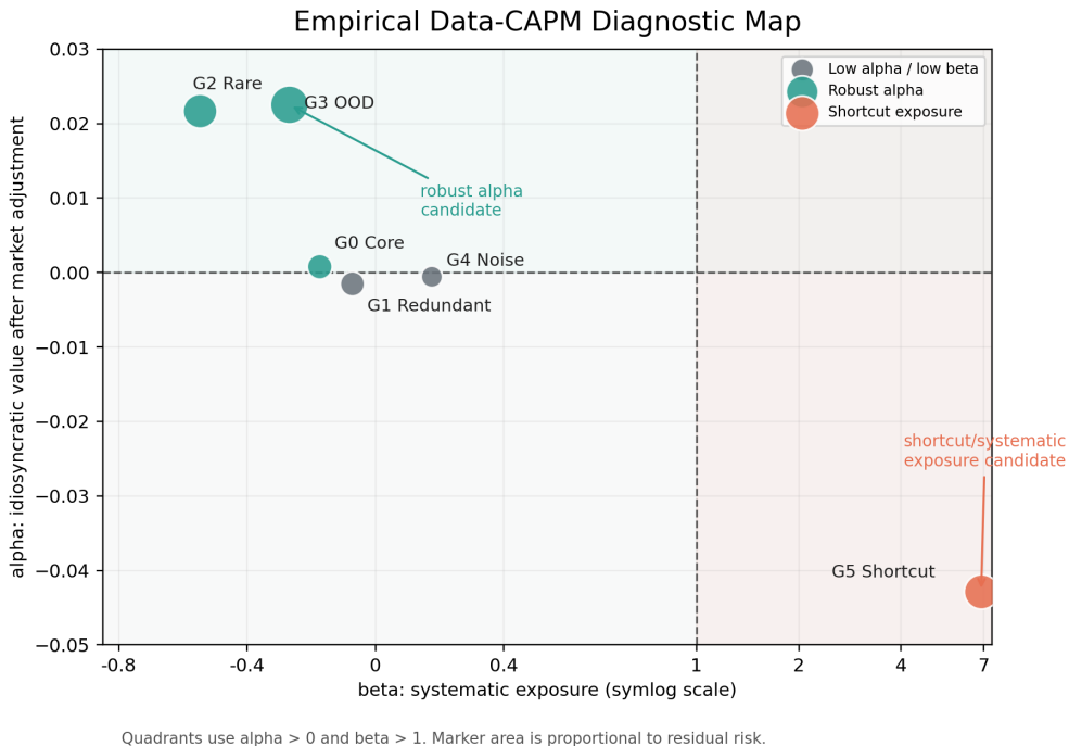
Figure 2: Empirical alpha-beta map on the synthetic benchmark. The x-axis uses a symmetric log scale so the high-beta shortcut and low-beta rare/OOD groups remain visible. Marker area is proportional to residual risk.
