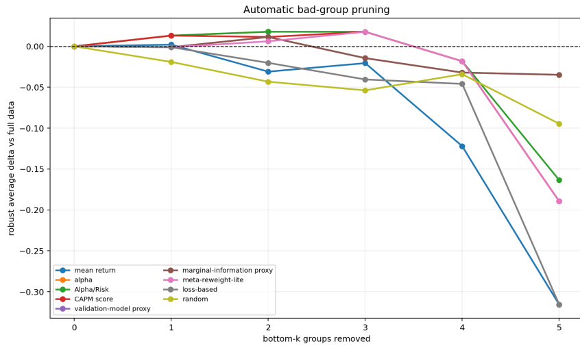
Figure 6: Synthetic pruning robust-average deltas. Pruning removes groups from low value to high value.
